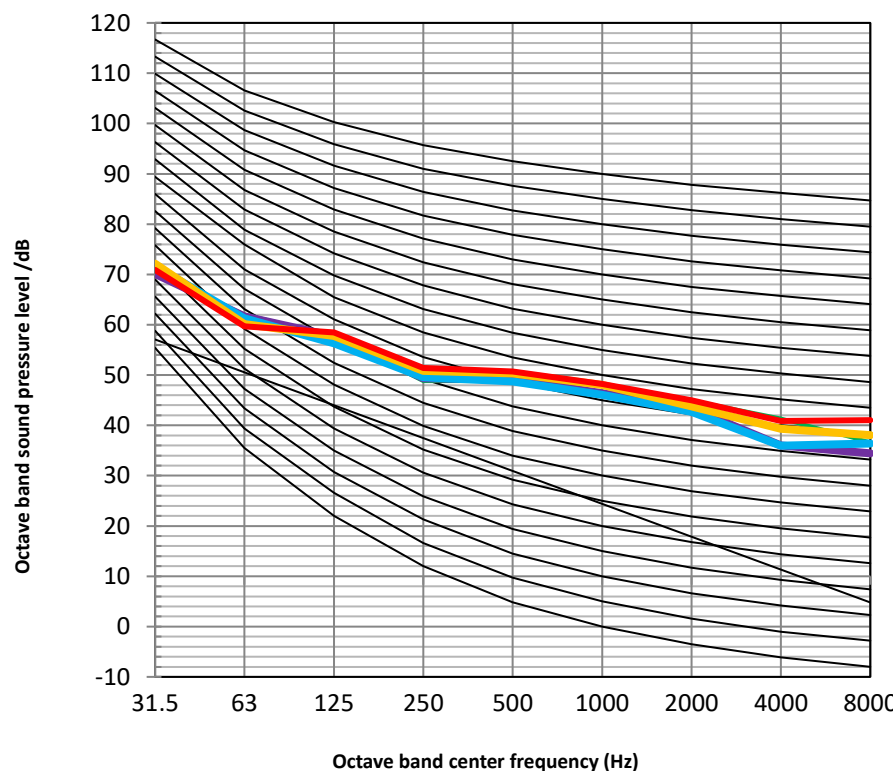
Figure 2-7.9: MDVC-V12WD2BR8-A(DE30/DB90) octave band levels
