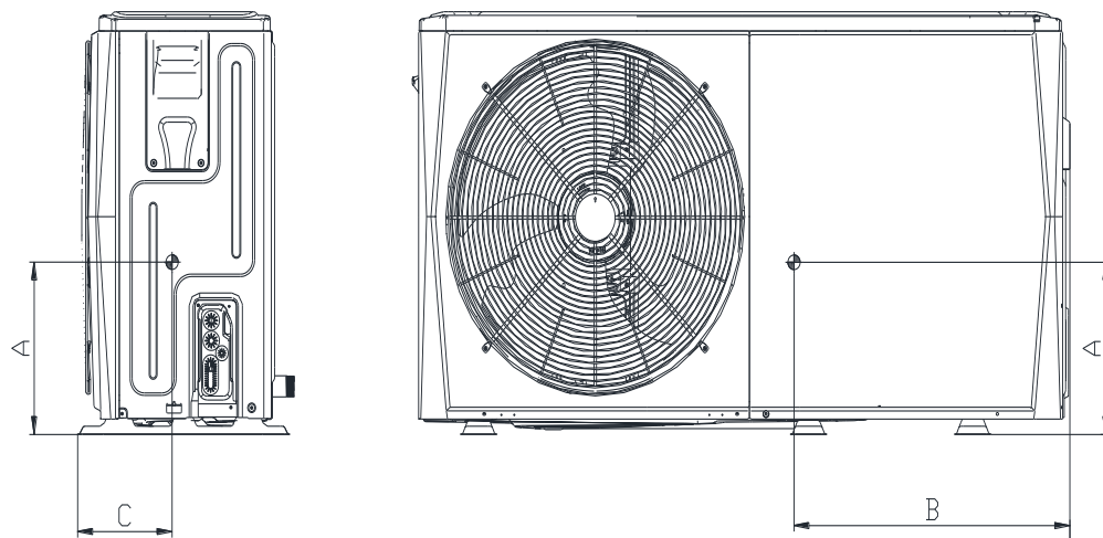
Figure 2-3.1: MDVC-V4(6)WD2ER8-A(DE30) dimensions and center of gravity (unit: mm)
