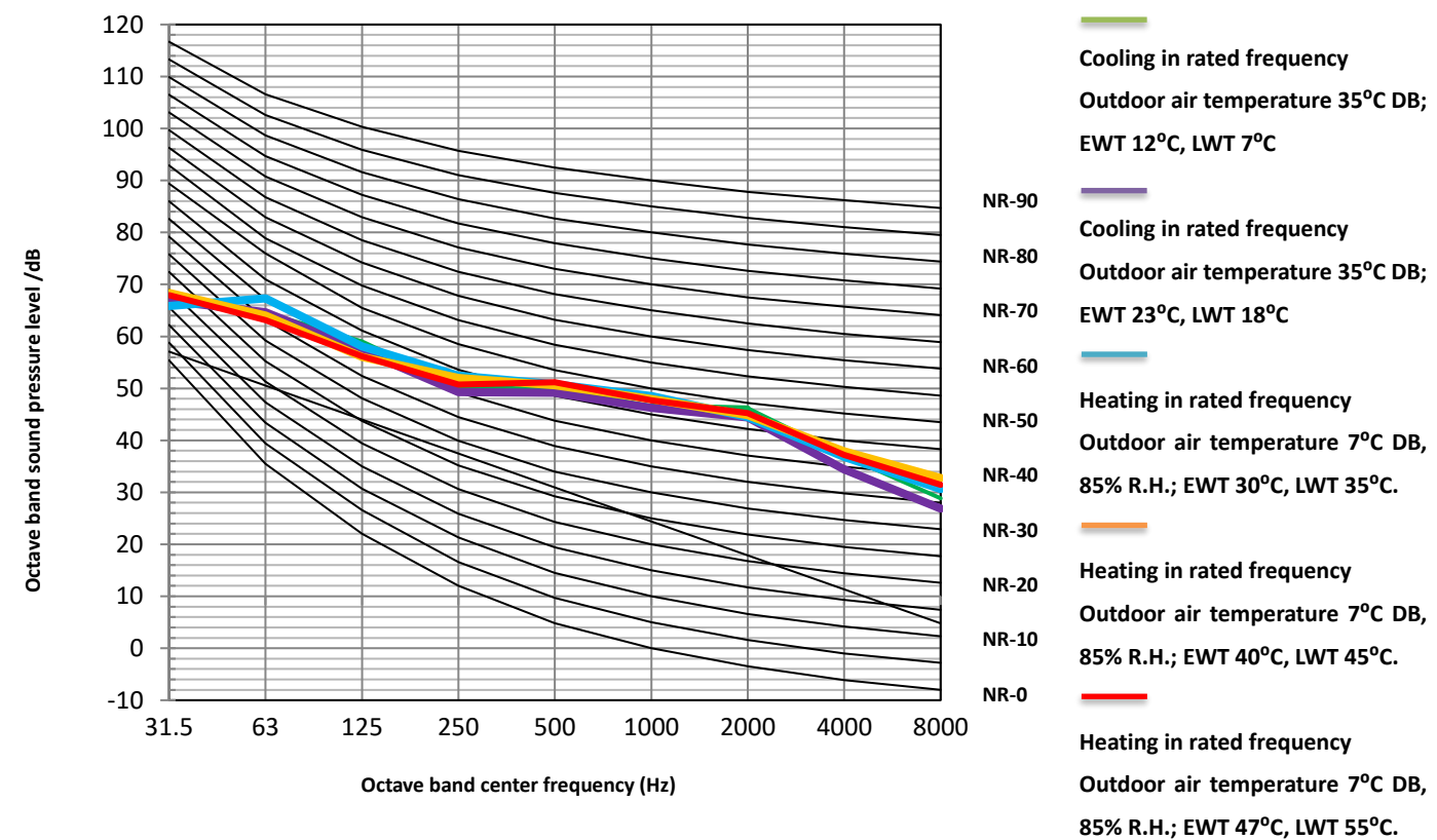
Figure 2-7.7: MDVC-V14WD2ER8-A(DE30/DB90) octave band levels
