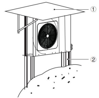
Figure 3-2.4: Snow shielding
