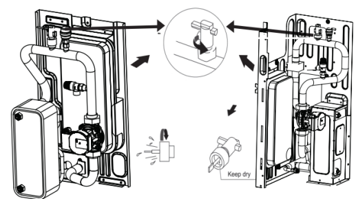
Figure 3-3.2: Water flow switch
