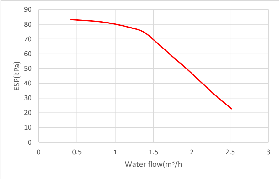
Figure 2-6.4: MDVC-V12(14,16)WD2E(B)R8-ADE30(DB90) hydronic performance 1
