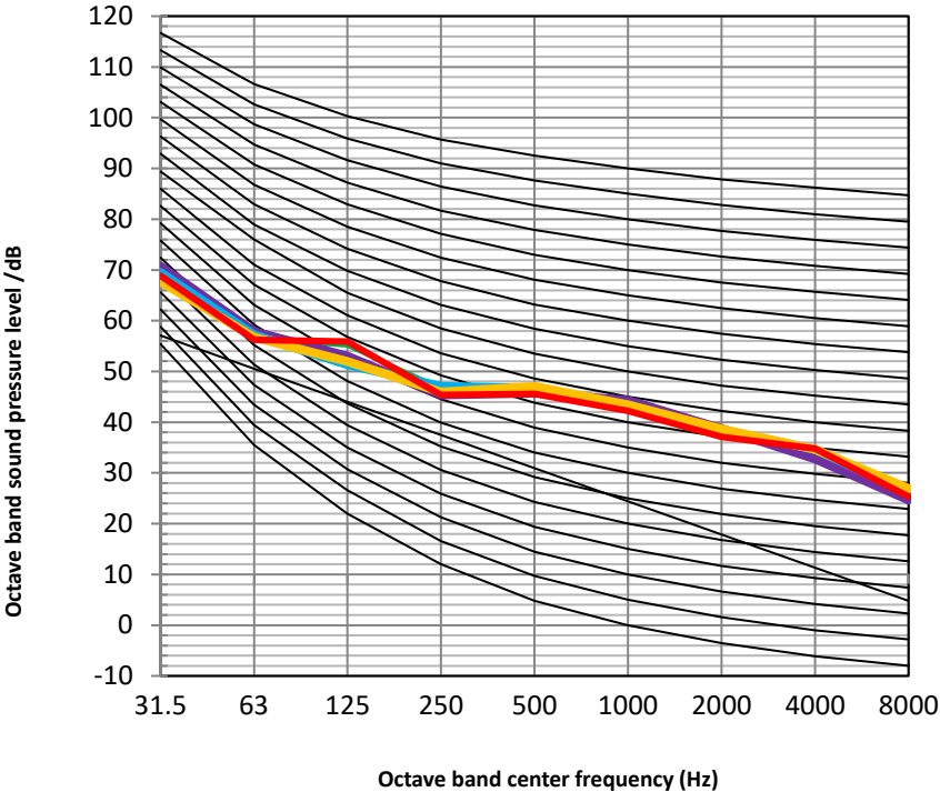
Figure 2-7.4: MDVC-V8WD2ER8-A(DE30/DB90) octave band levels
