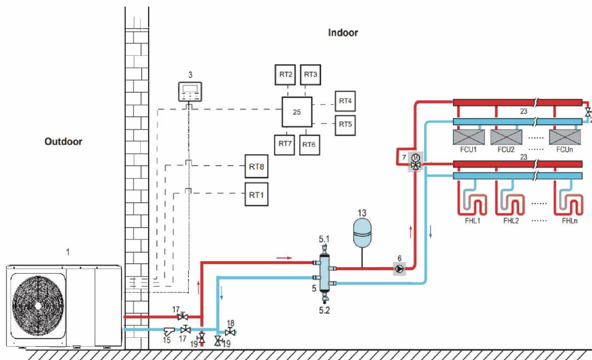
Figure 1-5.3: Application 2- Mode set control
