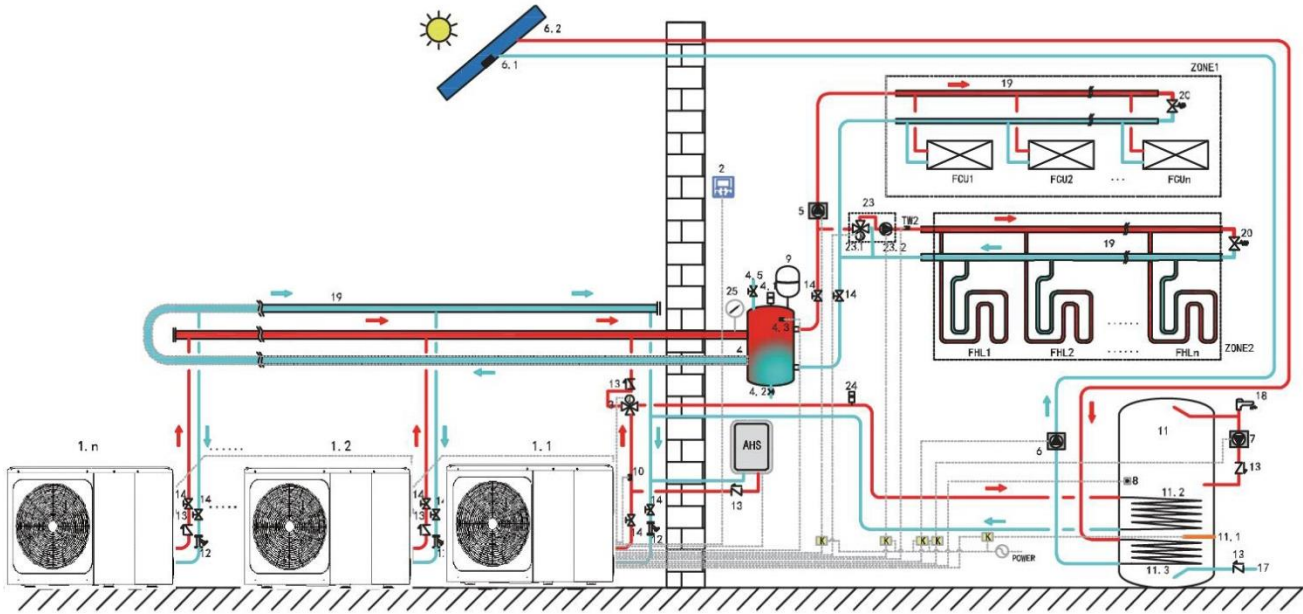
Figure 1-5.5: Application 3- Parallel system control
