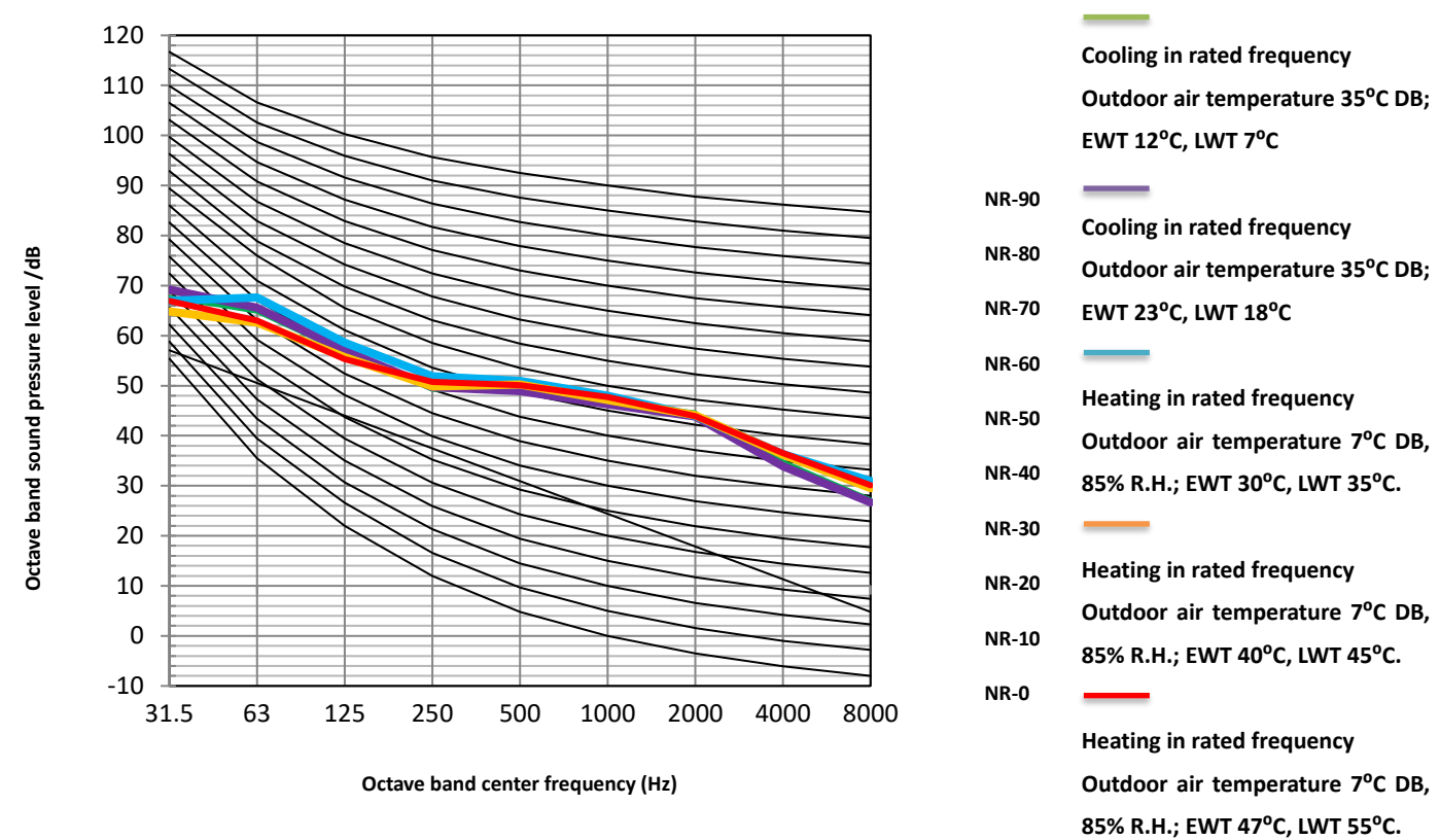
Figure 2-7.6: MDVC-V12WD2ER8-A(DE30/DB90) octave band levels
