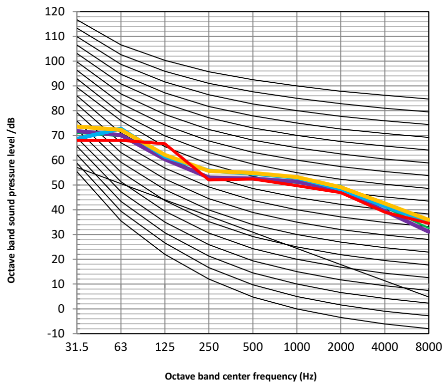
Figure 2-7.8: MDVC-V16WD2ER8-A(DE30/DB90) octave band levels
