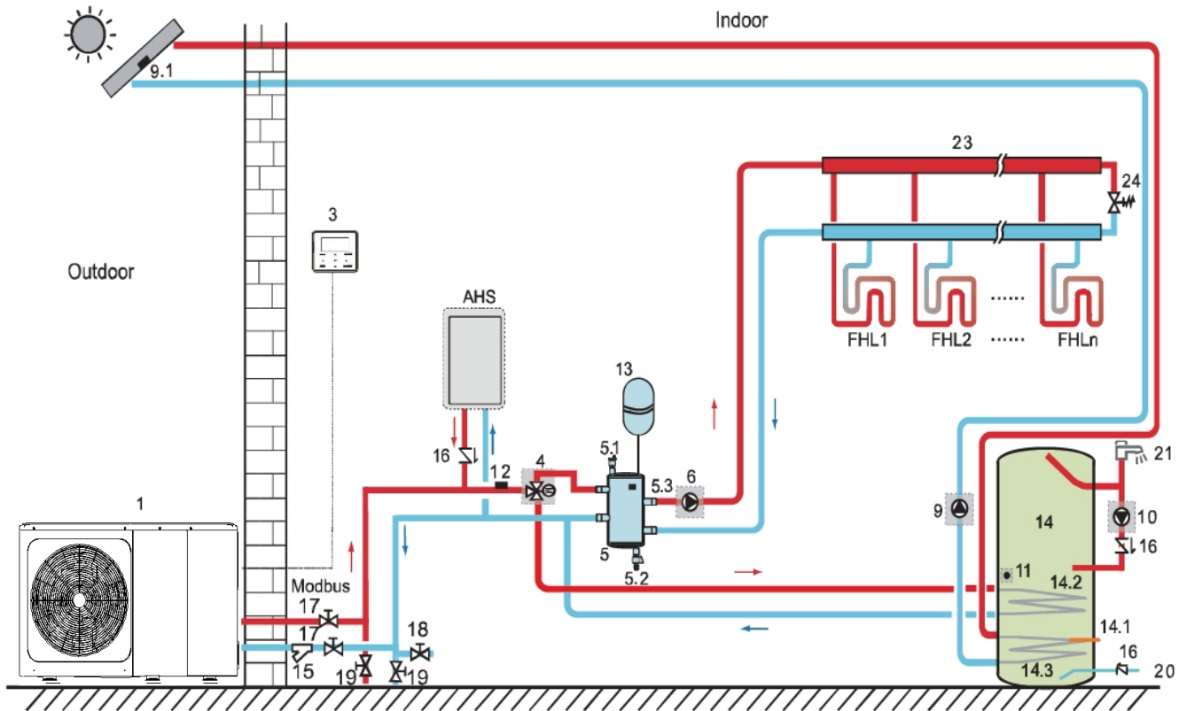
Figure 1-5.1: Application 1
