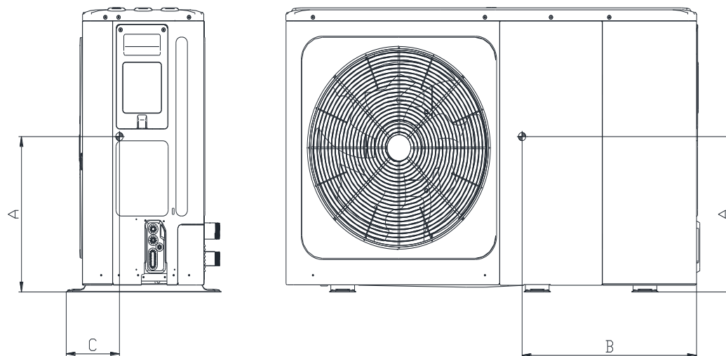
Figure 2-3.2: MDVC-V8(10)WD2ER8-A(DE30/DB90) MDVC-V12(14/16)WD2E(B)R8--A(DE30/DB90) dimensions and center of gravity (unit: mm)
