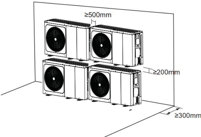
Figure 3-2.9: Installation with obstacles behind the unit
