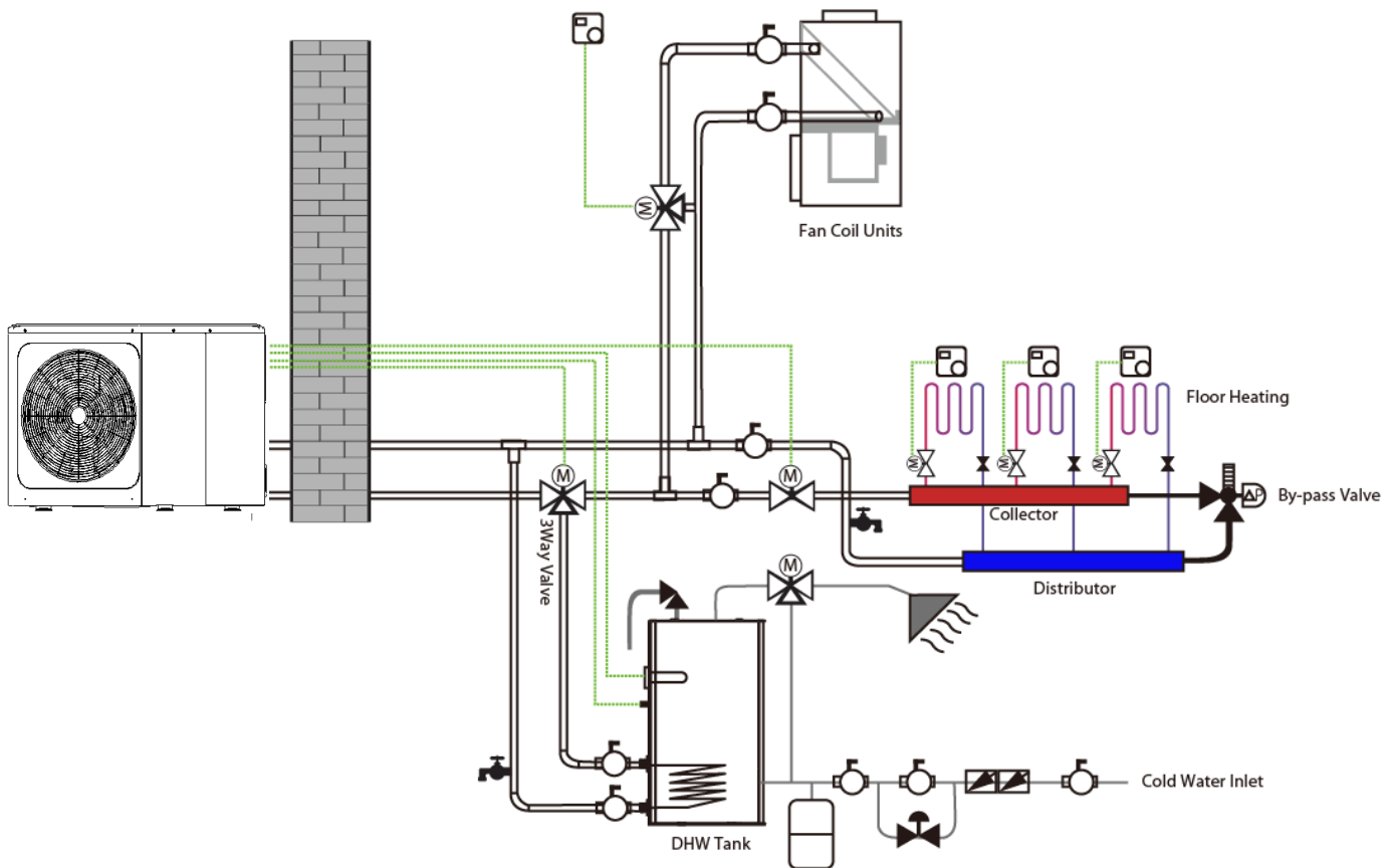
Figure 1-1.1: System schematic
