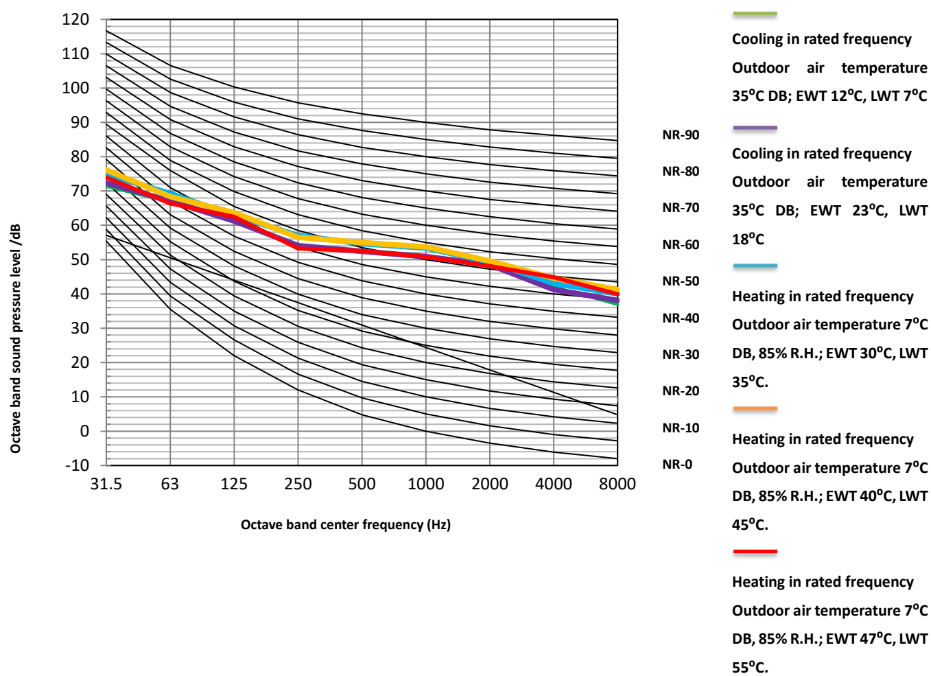
Figure 2-7.11: MDVC-V16WD2BR8-A(DE30/DB90) octave band levels
