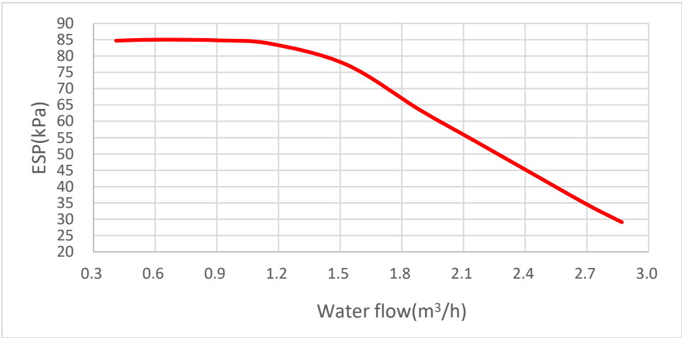
Figure 2-6.1: MDVC-V4(6, 8, 10)WD2ER8-A hydronic performance 1
