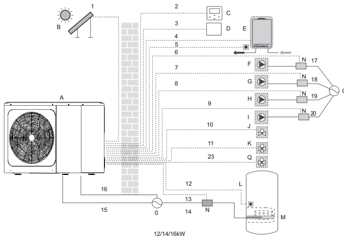
Figure 3-4.4: Wiring overview for 8/10/12/14/16kW models
