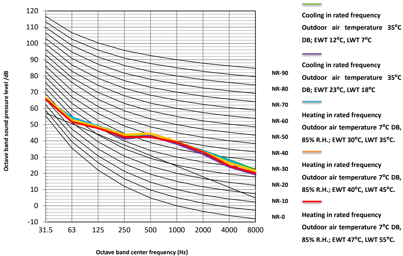
Figure 2-7.2: MDVC-V4WD2ER8-A(DE30) octave band levels
