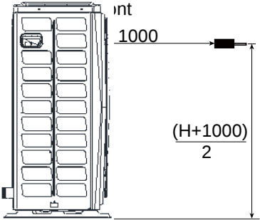
Figure 2-6.1: Sound pressure level measurement (unit: mm)
