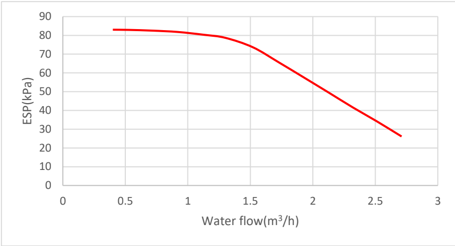
Figure 2-6.3: MDVC-V4(6, 8, 10)WD2ER8-ADE30 / MDVC-V8(10)WD2ER8-ADB90hydronic performance 1
