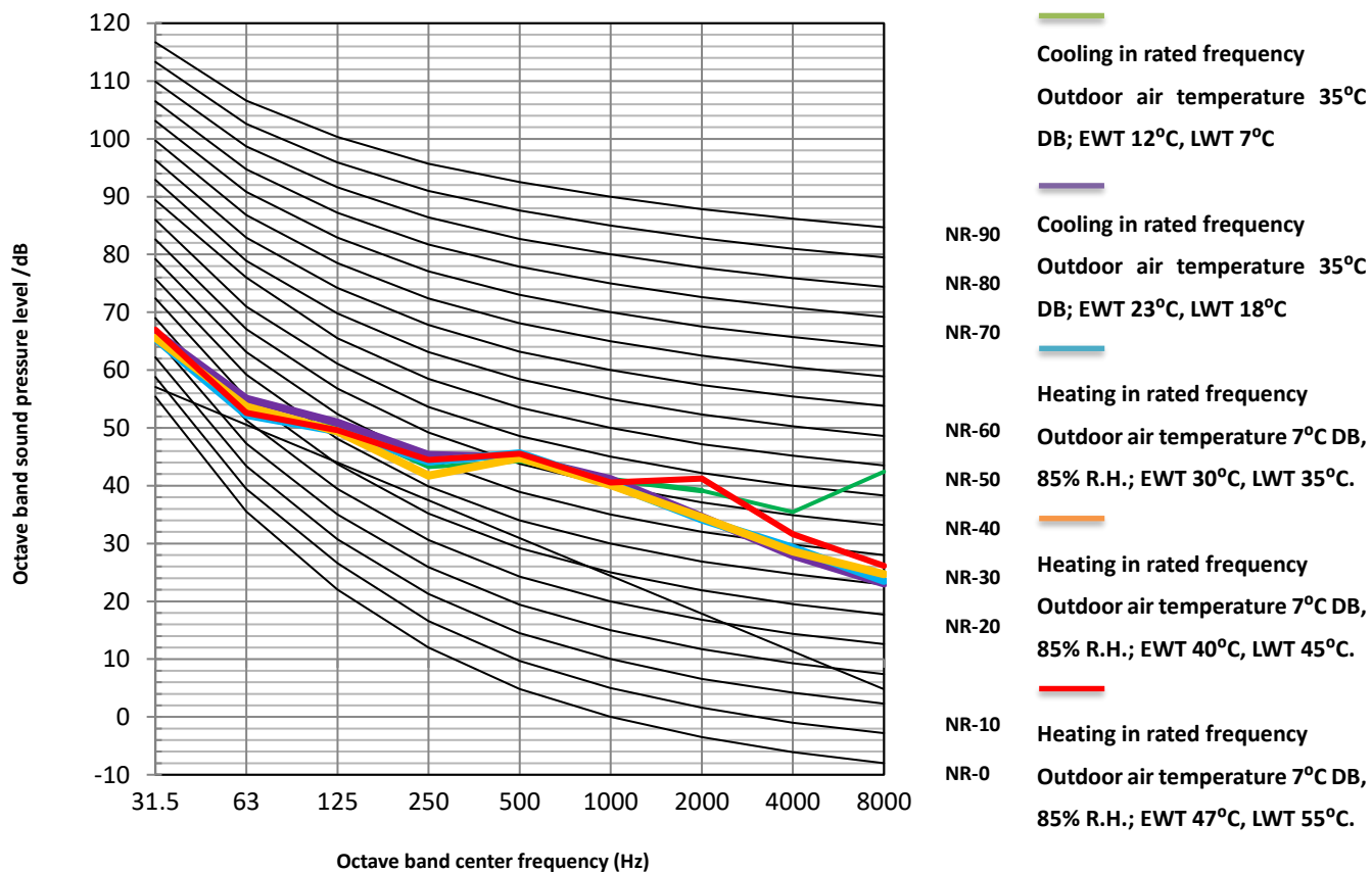
Figure 2-7.3: MDVC-V6WD2ER8-A(DE30) octave band levels
