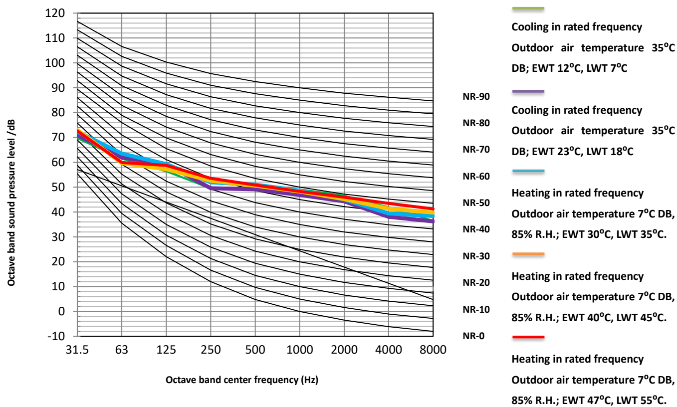
Figure 2-7.11: MDVC-V16WD2BR8-A(DE30/DB90) octave band levels
