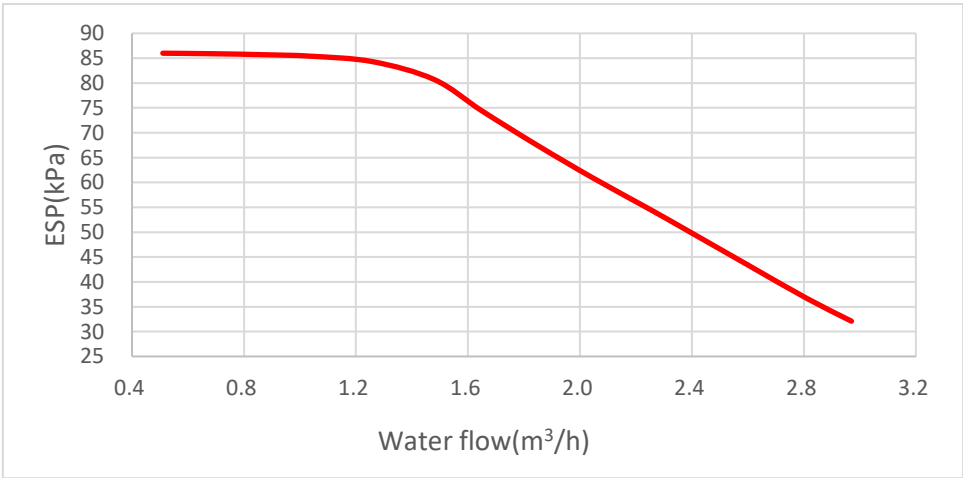
Figure 2-6.2: MDVC-V12(14, 16)WD2E(B)R8-A hydronic performance 1
