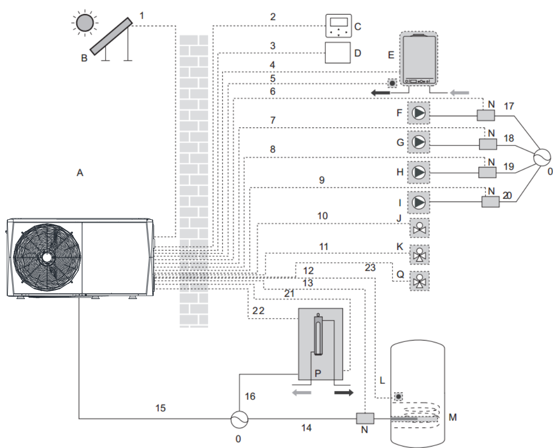
Figure 3-4.3: Wiring overview for 4/6kW models
