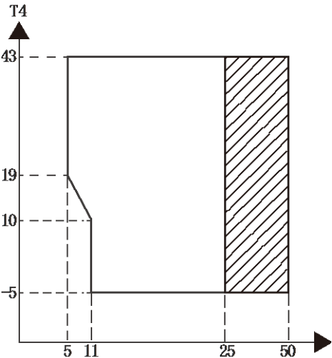
Figure 2-5.2: Cooling operating limits
