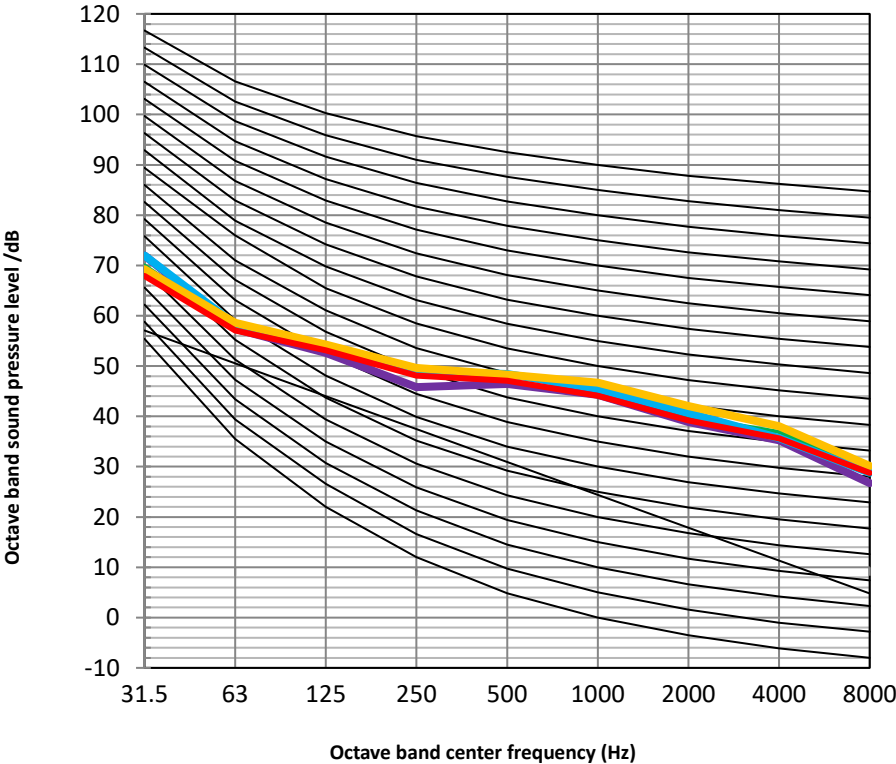
Figure 2-7.5: MDVC-V10WD2ER8-A(DE30/DB90) octave band levels
