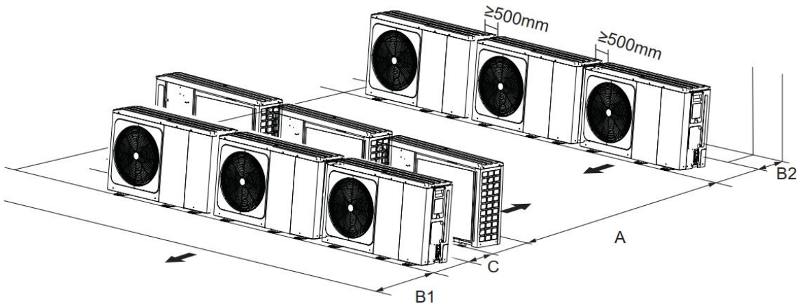
Figure 3-2.11: Multi-row installation
